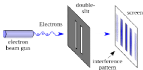
An illustration of the double-slit experiment in physics.
